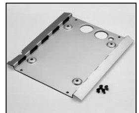
L4.73685.E Intermediate panel Zwischenblech
